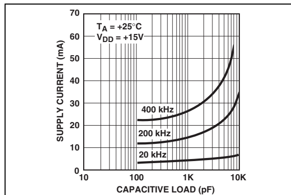
FIGURE 2-4: Supply Current vs. Capacitive Load.
