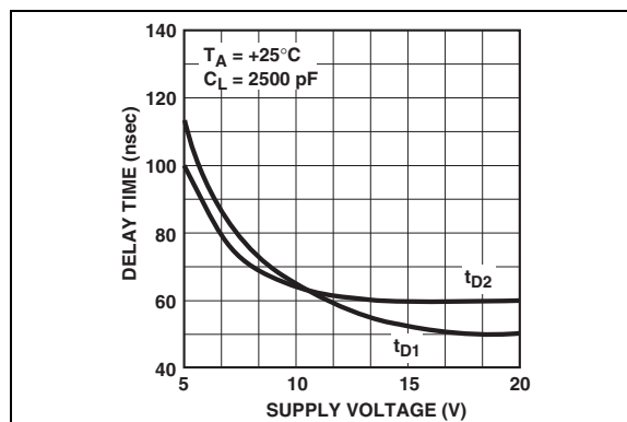
FIGURE 2-6: Delay Times vs. Supply Voltage.
