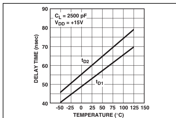
FIGURE 2-5: Delay Times vs. Temperature.
