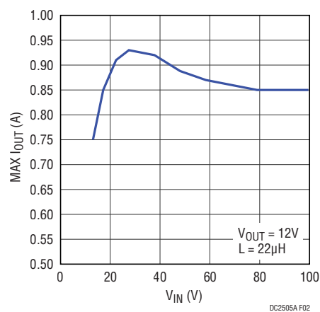
Figure 2. LT8630 Typical Maximum Load Current vs VIN
