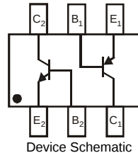
E1, B1, C1 = PNP4126 Section E2, B2, C2 = NPN4124 Section
