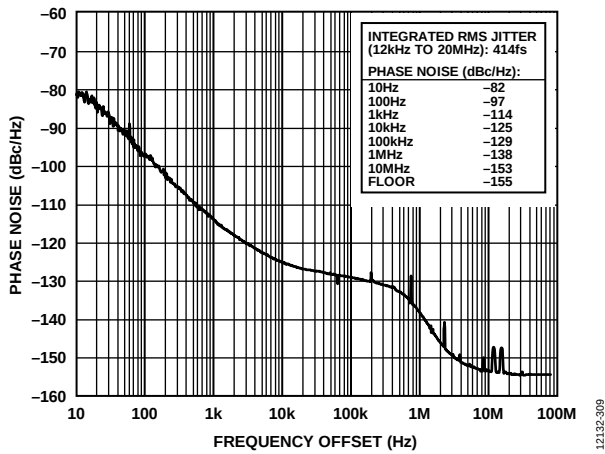
Figure 3. Absolute Phase Noise (Output Driver = 21 mA Mode), f_R = 19.44 MHz, f_{OUT} = 156.25 MHz, DPLL Loop Bandwidth = 50 Hz, f_{SYS} = 49.152 MHz Crystal
