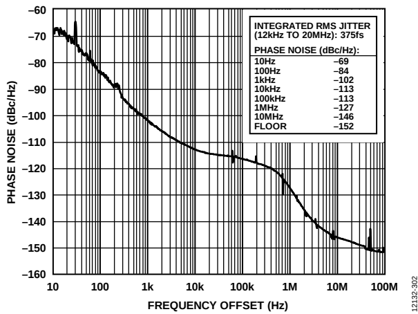
Figure 4. Absolute Phase Noise (Output Driver = 21 mA Mode), f_R = 19.44 MHz, f_{OUT} = 622.08 MHz, DPLL Loop Bandwidth = 50 Hz, f_{SYS} = 49.152 MHz Crystal
