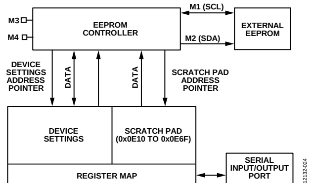
Figure 32. EEPROM Functional Diagram
