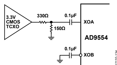
Figure 25. System Clock Input (XOA, XOB) When Using a TCXO/OCXO with 3.3 V CMOS Output
