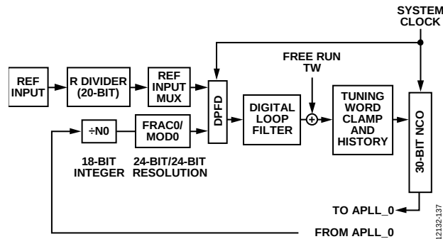
Figure 27. DPLL_0 Core
