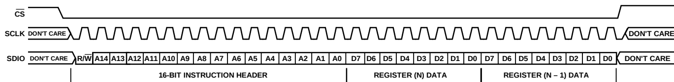
Figure 33. Serial Control Port Write—MSB First, Address Decrement, Two Bytes of Data
