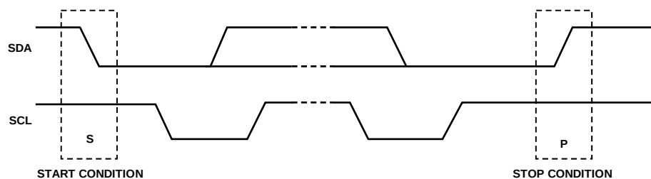
Figure 40. Start and Stop Conditions
