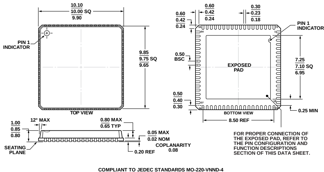
Figure 45. 72-Lead Lead Frame Chip Scale Package [LFCSP_VQ] 10 mm × 10 mm Body, Very Thin Quad (CP-72-4) Dimensions shown in millimeters
