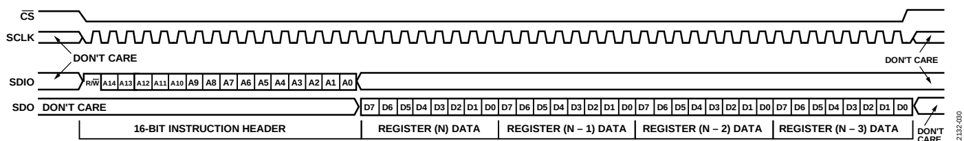
Figure 34. Serial Control Port Read—MSB First, Address Decrement, Four Bytes of Data
