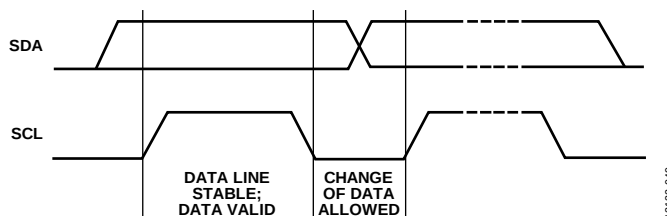
Figure 39. Valid Bit Transfer
