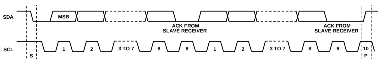
Figure 41. Acknowledge Bit
