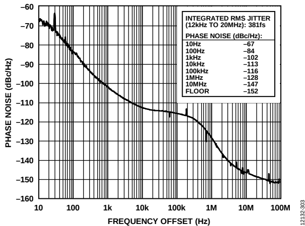
Figure 5. Absolute Phase Noise (Output Driver = 21 mA Mode), f_R = 19.44 MHz, f_{OUT} = 644.53125 MHz, DPLL Loop Bandwidth = 50 Hz, f_{SYS} = 49.152 MHz Crystal
