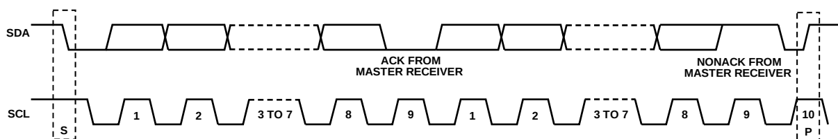
Figure 43. Data Transfer Process (Master Read Mode, 2-Byte Transfer), First Acknowledge From Slave
