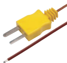
80PK-1 General Purpose Bead Temperature Probe
