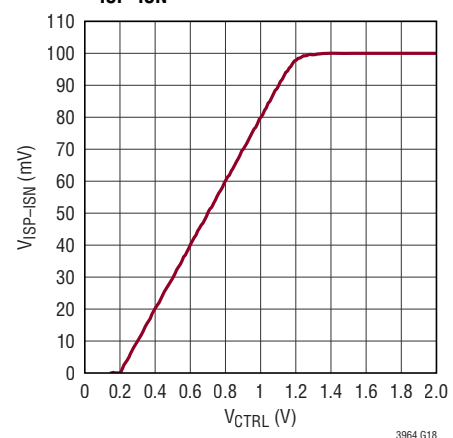
V_{ISN-10N} vs V_{CTRL}
