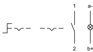
Wiring diagram 17
