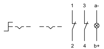
Wiring diagram 18
