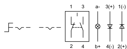
Wiring diagram 21
