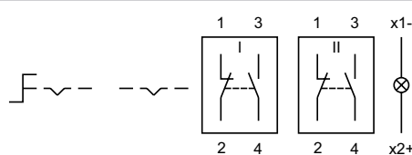
Wiring diagram 26
