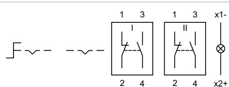
Wiring diagram 26
