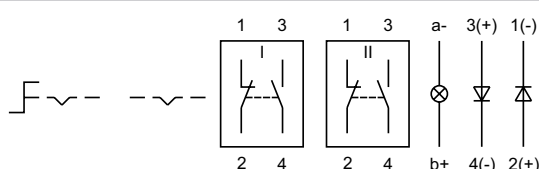
Wiring diagram 25
