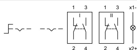
Wiring diagram 26
