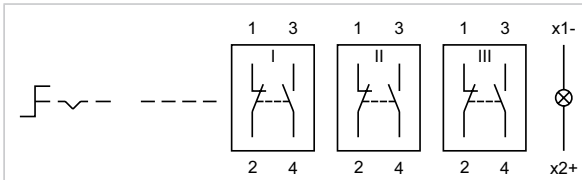
Wiring diagram 13
