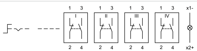
Wiring diagram 14
