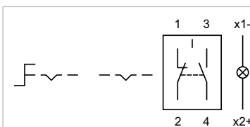
Wiring diagram 22
