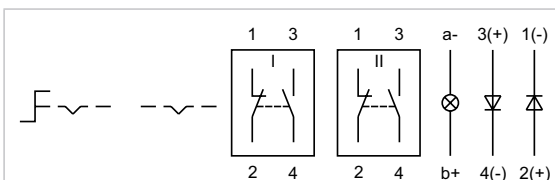
Wiring diagram 25
