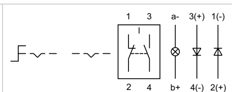
Wiring diagram 21
