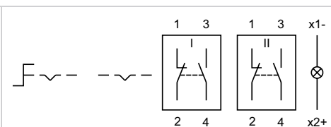
Wiring diagram 26
