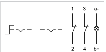
Wiring diagram 18
