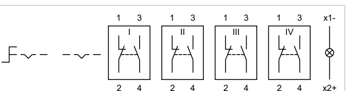
Wiring diagram 28
