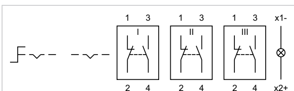
Wiring diagram 27
