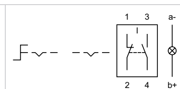
Wiring diagram 23
