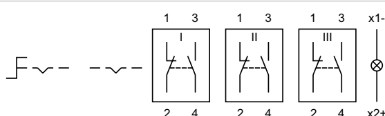
Wiring diagram 27
