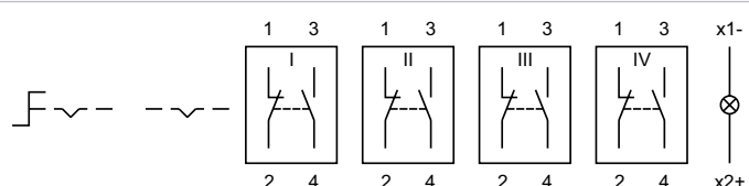
Wiring diagram 28
