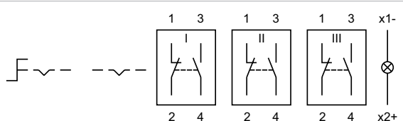
Wiring diagram 27
