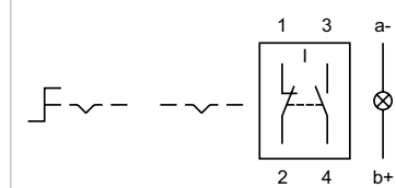
Wiring diagram 23
