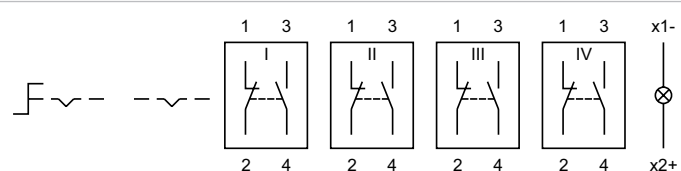
Wiring diagram 28
