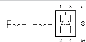
Wiring diagram 23
