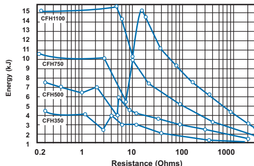
Absorbed energy for wire temperature of 500°C (Impulse time ≤ 0,2")
