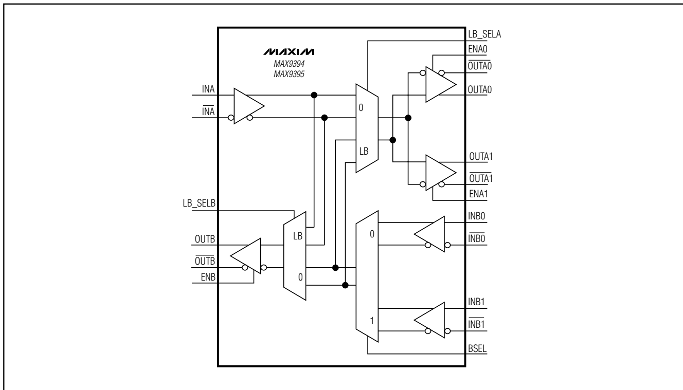
Functional Diagram
