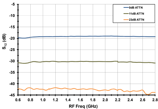
S 12 (device+C5 cap) [ T_{AMB} = 25C , V_{CC} = 5.00 Volts]
