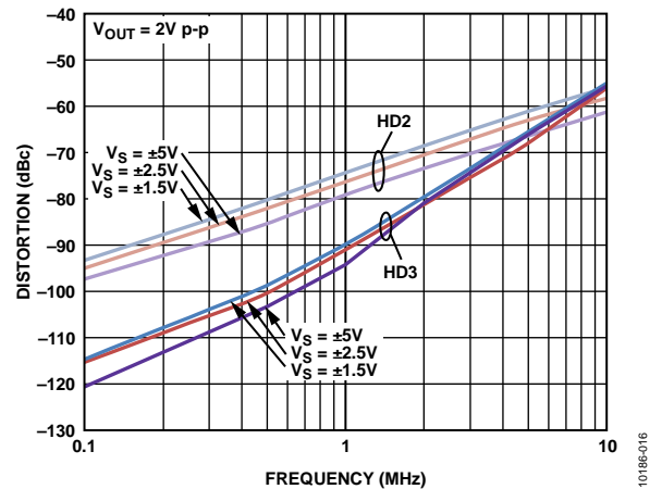
Figure 19. Harmonic Distortion vs. Frequency for Various Supplies
