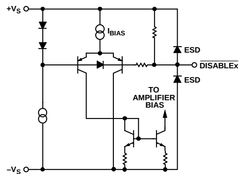
Figure 45. \overline{\text{DISABLEx}} Circuit
