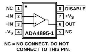
Figure 1. ADA4895-1 Single Amplifier (8-Lead SOIC)
