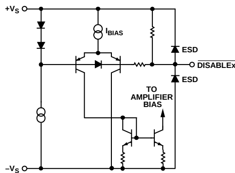
Figure 45. DISABLEx Circuit
