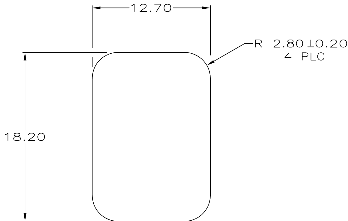
SOCKET HOUSING CUT OUT
