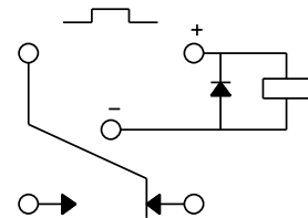
TERMINAL VIEW
