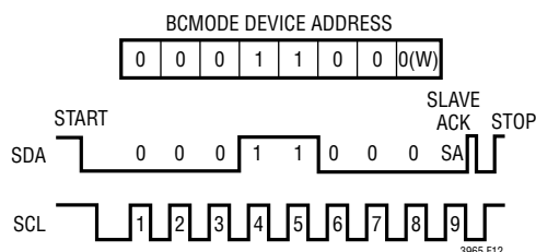
Figure 12. LT3965/LT3965-1 I²C Serial Port BCMODE Write Protocol
