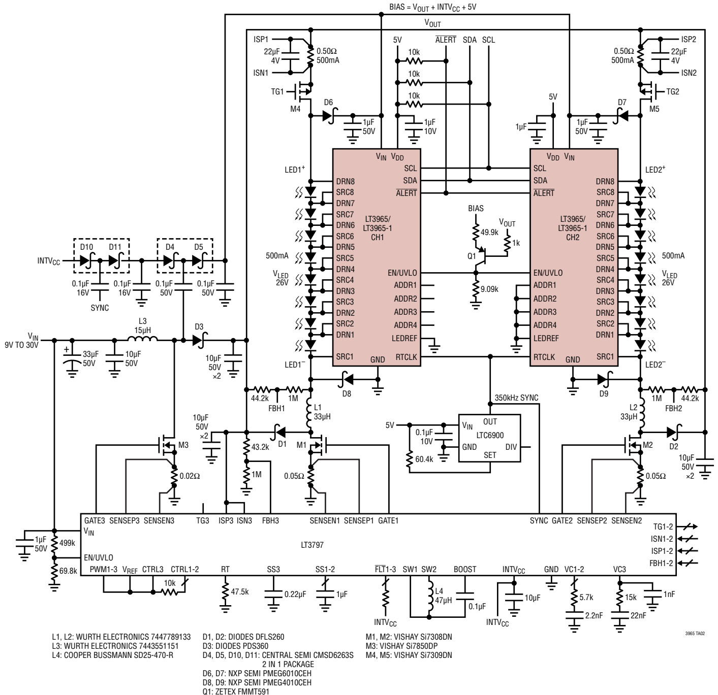
Matrix LED Dimmer Powered by a Dual Buck Mode LED Driver with a Boost Pre-Regulator
