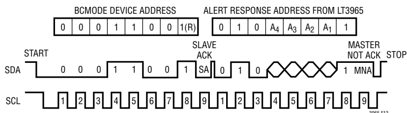
Figure 13. LT3965/LT3965-1 I²C Serial Port BCMODE Read Protocol
