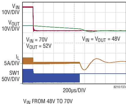
Pass-Thru Positive Surge (Falling Edge)
