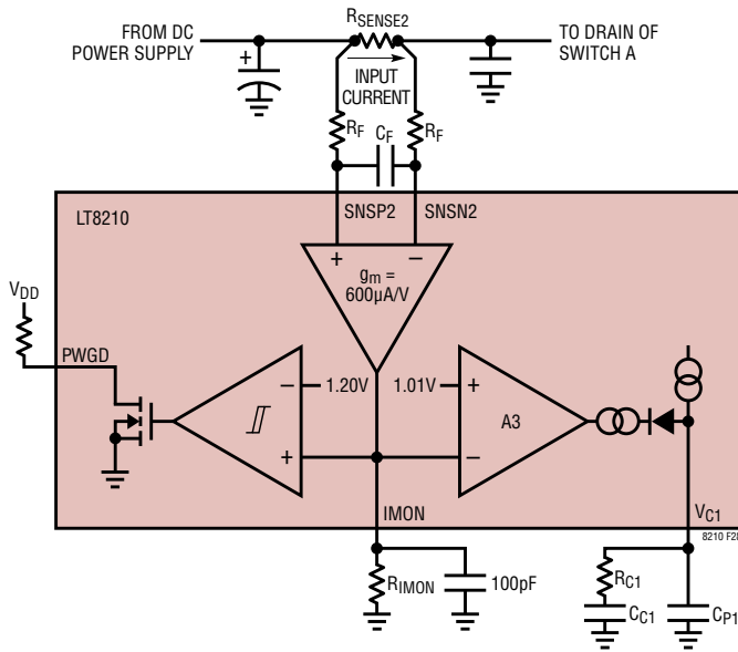
Figure 28. Input Current Monitor and Limit Using Input Filter
