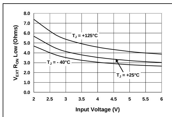
FIGURE 2-30: V_{EXT} Low Output Voltage vs. Input Voltage.
