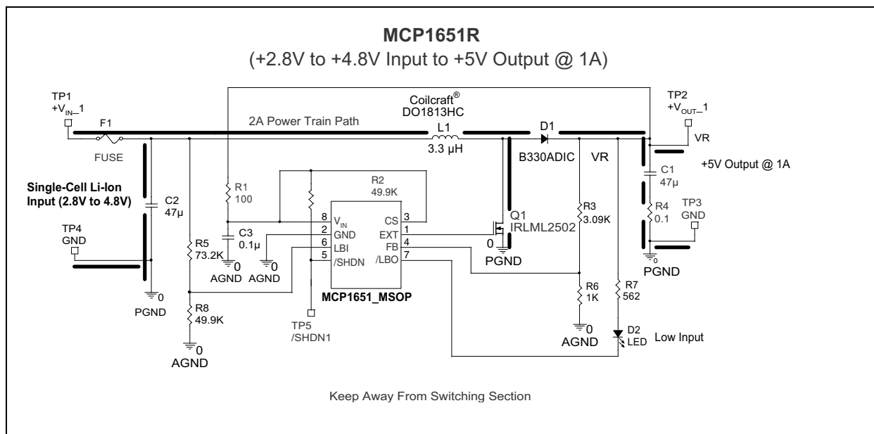
FIGURE 6-1: MCP1650/51/52/53 Application Schematic.
