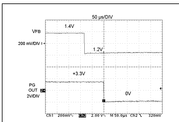
FIGURE 2-27: PG Timing.
