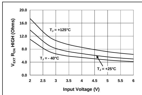
FIGURE 2-29: V_{EXT} High Output Voltage vs. Input Voltage.
