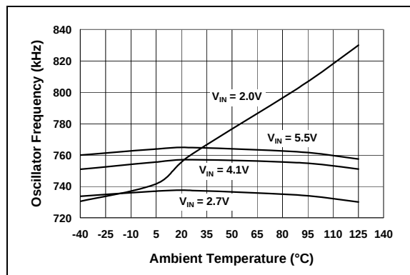
FIGURE 2-4: Oscillator Frequency vs. Ambient Temperature.
