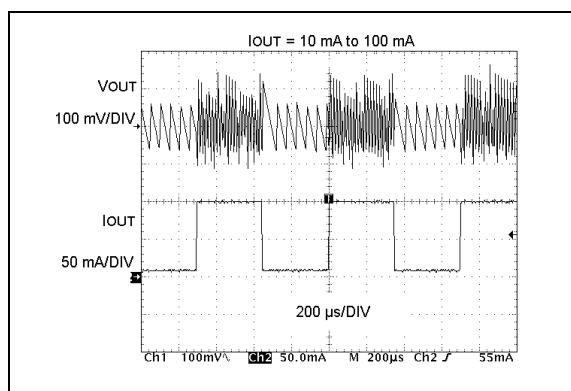
FIGURE 2-12: Dynamic Load Response.
