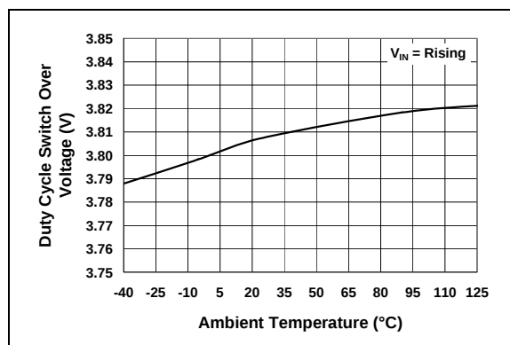
FIGURE 2-5: Duty Cycle Switch-Over Voltage vs. Ambient Temperature.
