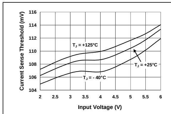
FIGURE 2-28: Current Sense Threshold vs. Input Voltage.
