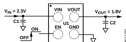
Figure 1. ADP172 with Fixed Output Voltage, 1.8 V
