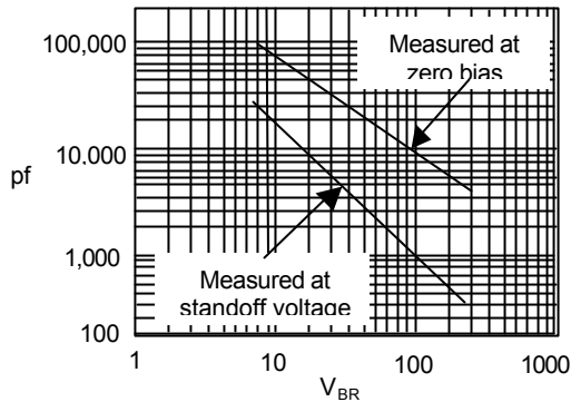
Figure 3 - Typical Capacitance
