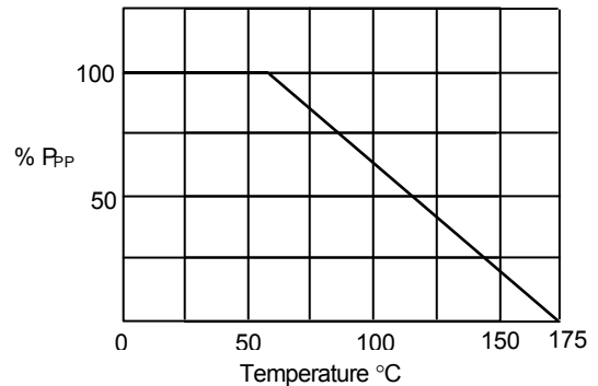
Figure 4 - Derating Curve
