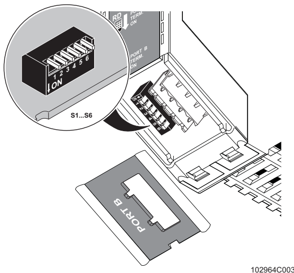
Figure 4 DIP switches
