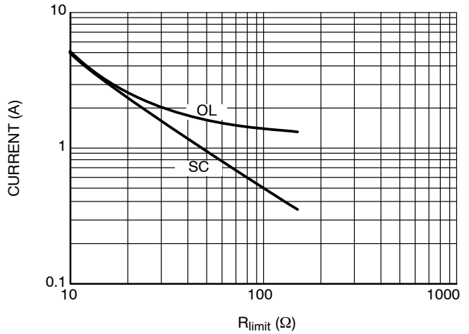
Figure 13. Current Limit vs. R_{\text{sense}} for Direct Current Sensing
