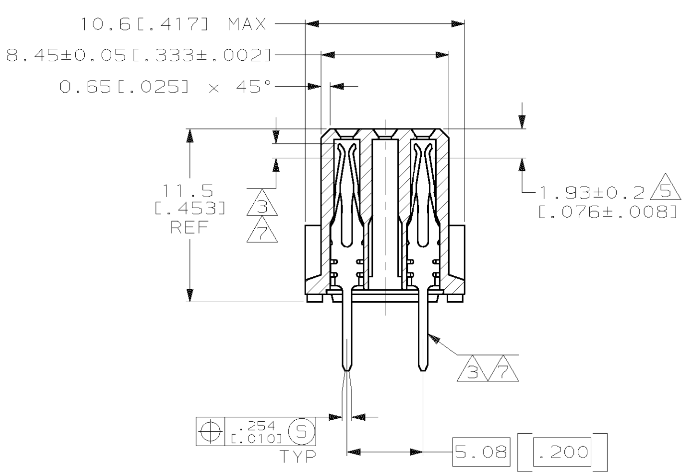
SECTION X-X
