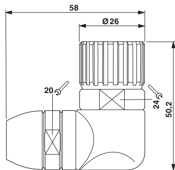
Dimensional drawing
