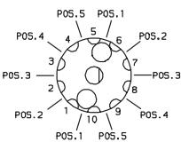
DP MODELS 36° INDEXING SCHEMATIC
