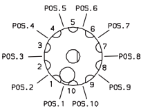
SP MODELS 36° INDEXING SCHEMATIC
