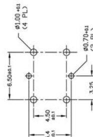
P.C. MOUNTING
