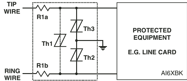
Figure 15. Protection Module
