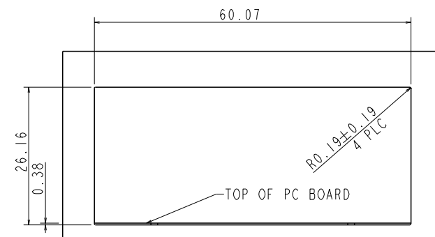
SUGGESTED PANEL CUTOUT DIMENSIONS
