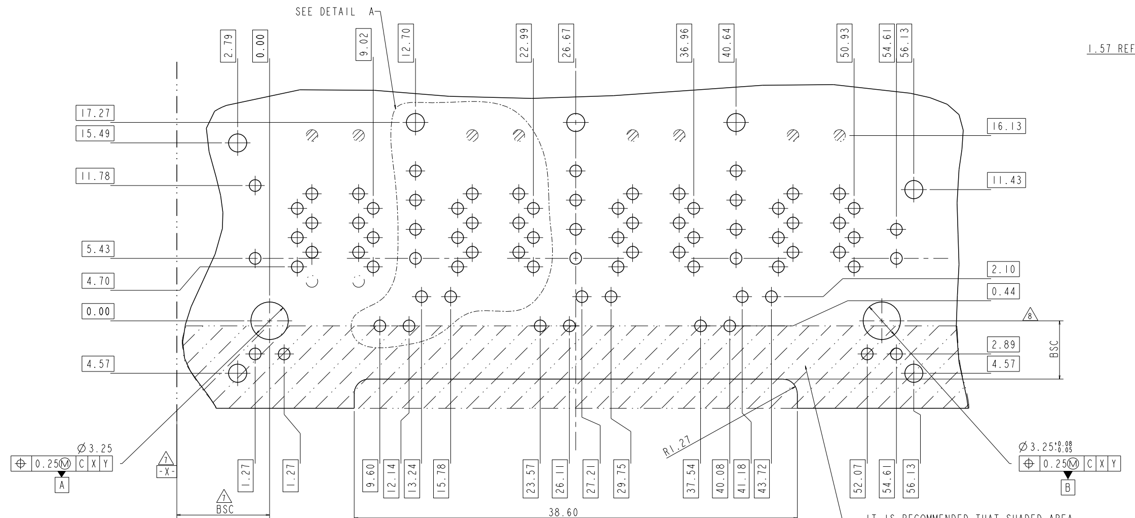
PC BOARD LAYOUT VIEWED FROM COMPONENT SIDE SCALE 6:1
