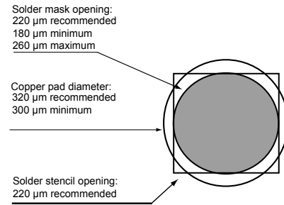
Figure 15. Footprint - 3 mils stencil - solder mask defined
