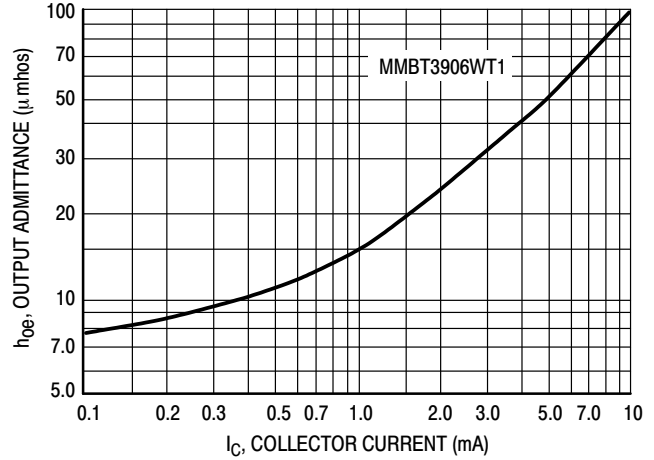
Figure 29. Output Admittance
