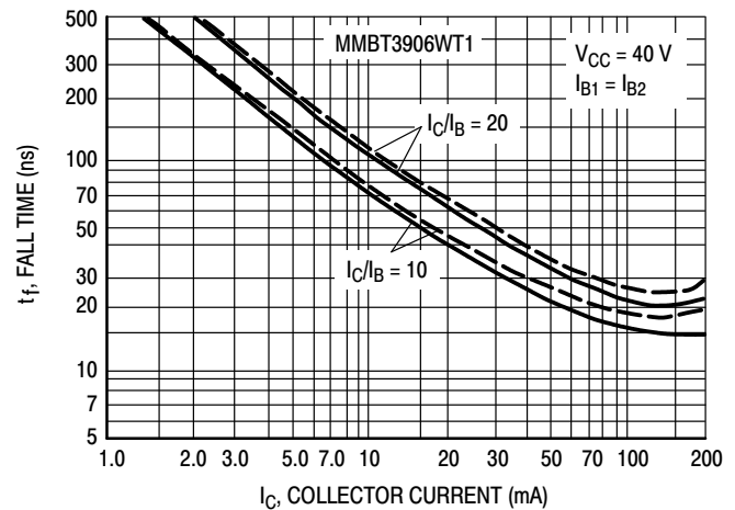
Figure 25. Fall Time
