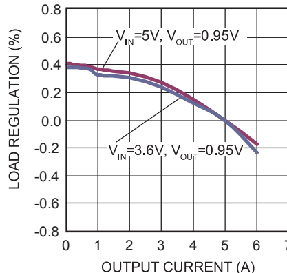
Load Regulation Vs. I_{OUT}
