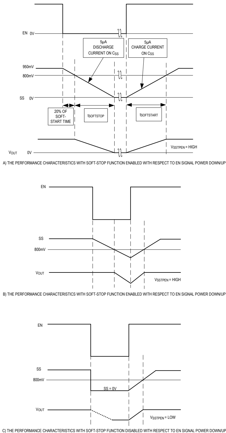
Figure 4. Soft-Stop Function Timing Diagram
