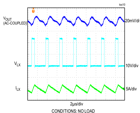
STEADY-STATE SWITCHING WAVEFORMS (5V OUTPUT, PWM MODE, FIGURE 8 CIRCUIT)
