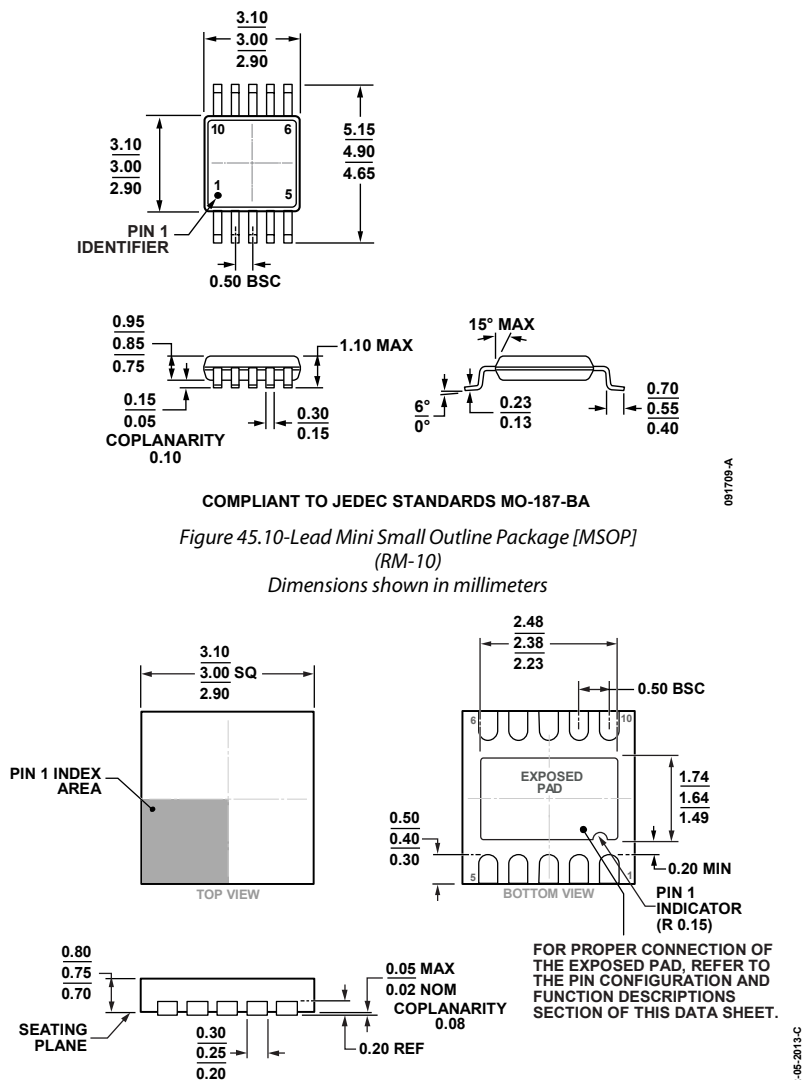
Figure 46. 10-Lead Lead Frame Chip Scale Package [LFCSP] 3 mm x 3 mm Body and 0.75 mm Package Height (CP-10-9)
