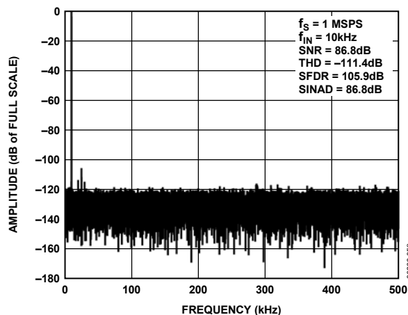
Figure 11. FFT Plot, REF = 2.5 V
