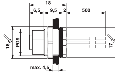
M12 flush-type connector
