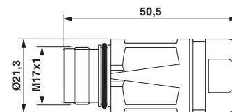
Dimensioned drawing
