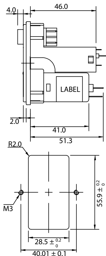
PANEL CUTOUT (MOUNTING FROM FRONT)
