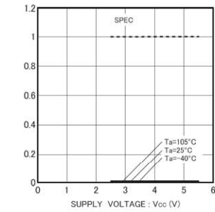
Fig.38 Input leak current ILI(CS,SK,DI)
