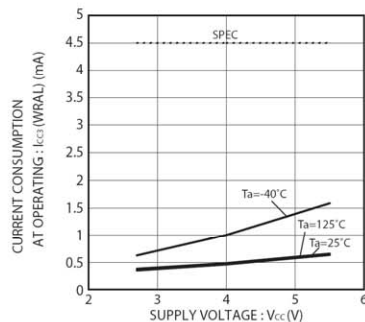
Fig.12 Consumption current at WRAL operation I_{CC3} (WRAL, f_{SK}=1.25\text{MHz} )
