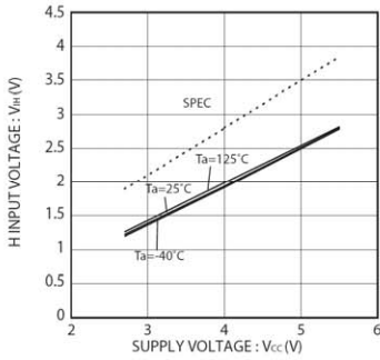
Fig.2 H input voltage V_{IH} (CS,SK,DI)
