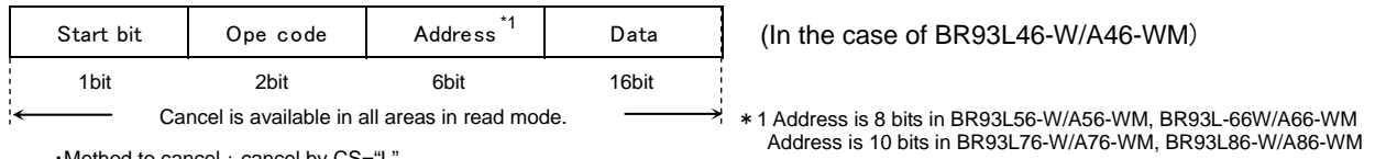
Fig.66 READ cancel available timing
