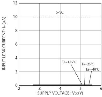
Fig.8 Input leak current I_{LI} (CS,SK,DI)
