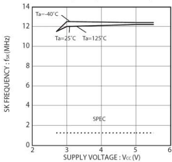
Fig.14 SK frequency f_{SK}
