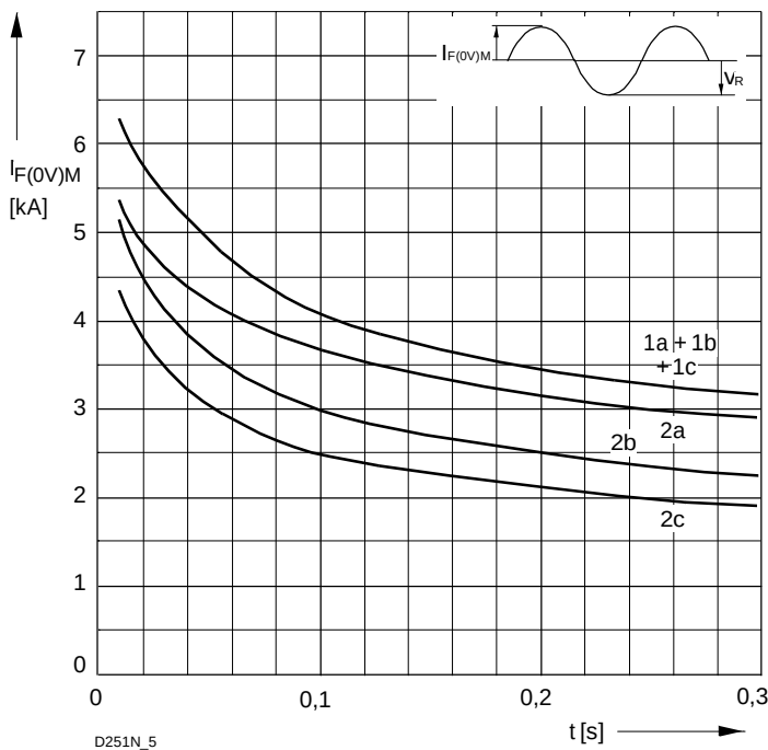
Bild / Fig. 3 Grenzstrom / Maximum overload forward current I_{F(0V)M} = f(t) 1 - I_{FAV(vor)} = 0\text{ A} ; t_j = t_c = 25\text{ °C} 2 - I_{FAV(vor)} = 250\text{ A} ; t_c = 130\text{ °C} ; t_j = 180\text{ °C} a - V_R \leq 50\text{ V} b - V_R = 0,5 V_{RRM} c - V_R = 0,8 V_{RRM}
