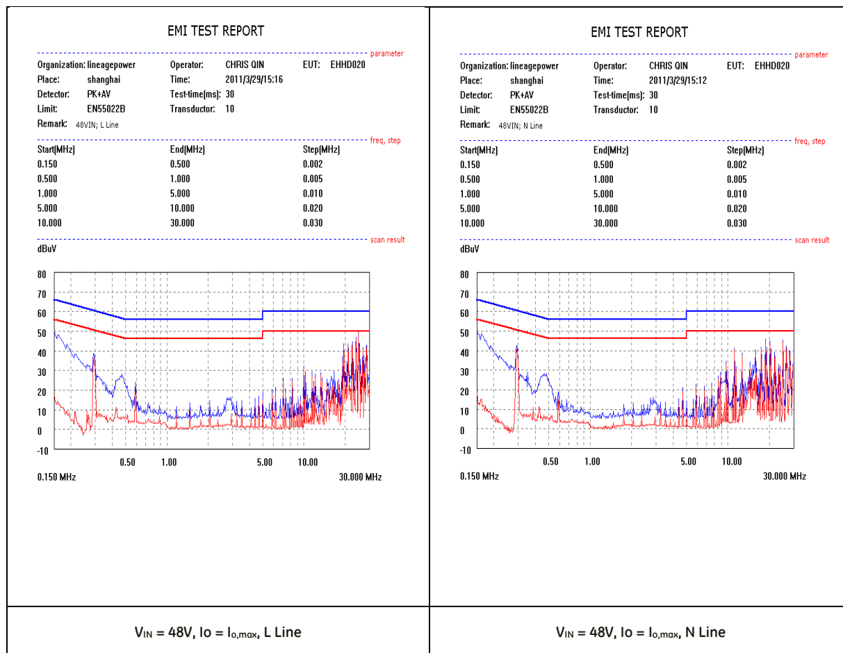
Figure 29. EMC Considerations
